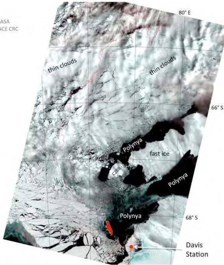
Figure 1: MODIS image, acquired 10/11/2013 and provided by NASA.
