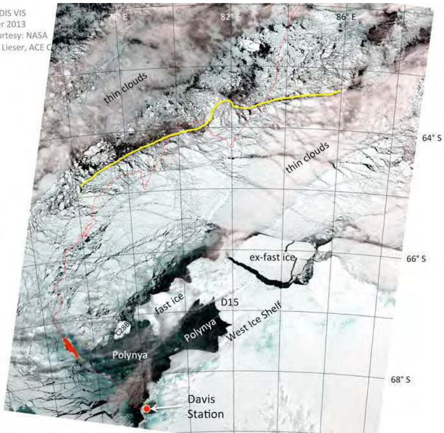
Figure 1: MODIS image, acquired 06/11/2013 and provided by NASA.
