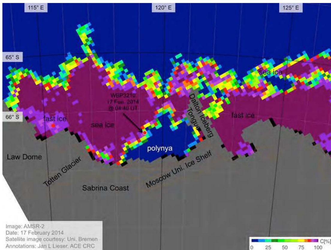
Figure 4: AMSR-2 image, acquired 17/02/2014 and provided by Universität Bremen.
