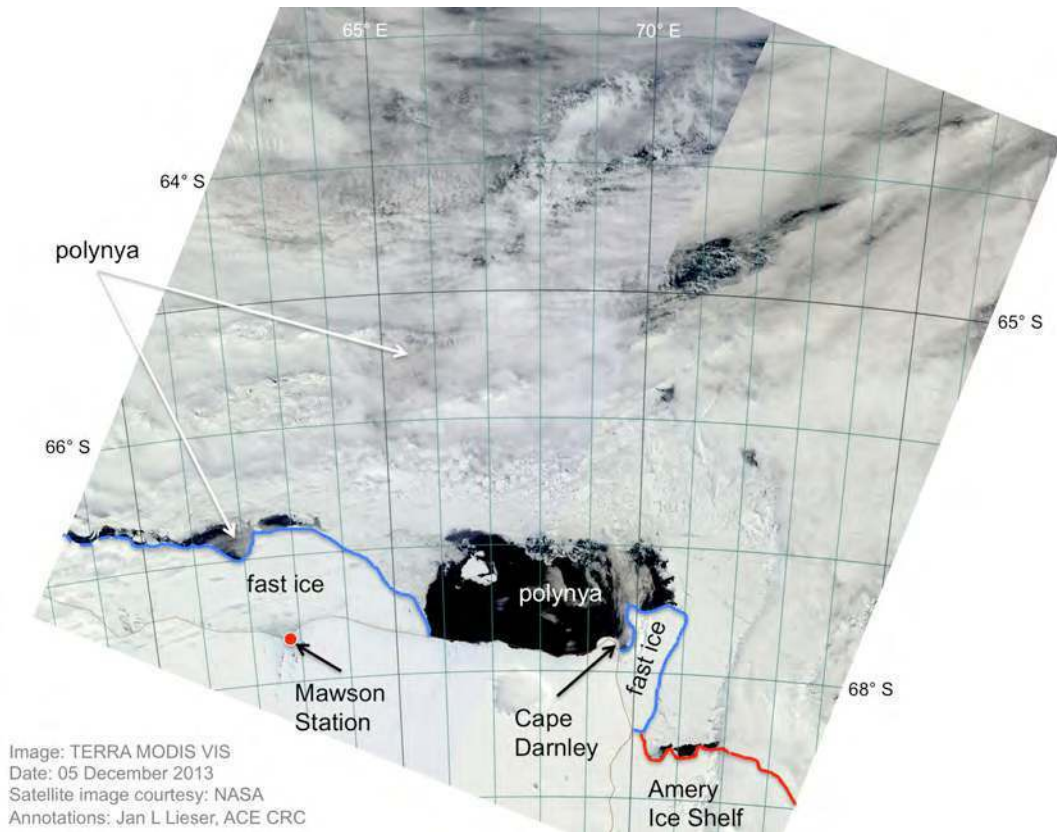
Figure 1: MODIS image, acquired 05/12/2013 and provided by NASA.
