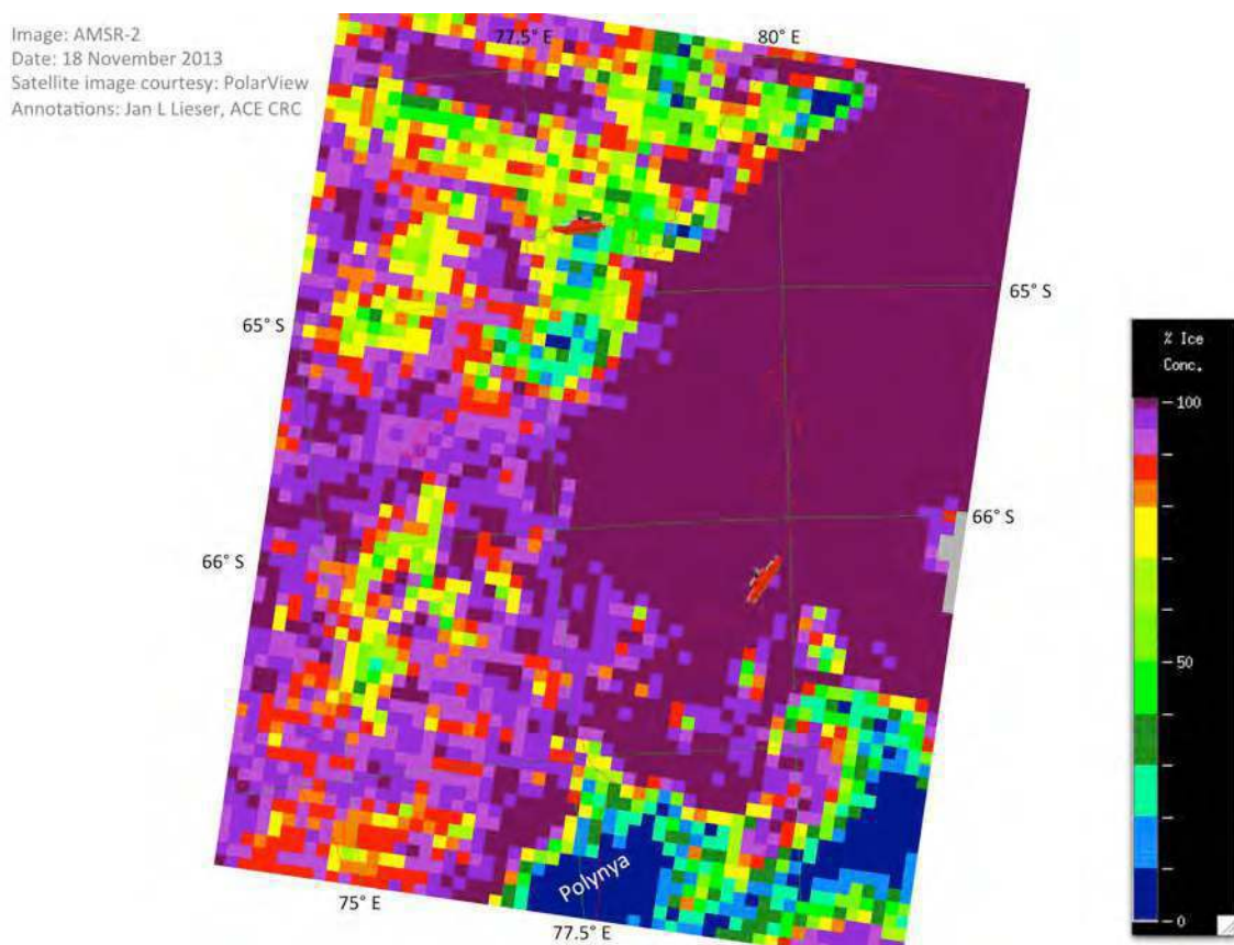
Figure 1: AMSR-2 image, acquired 18/11/2013 and provided by PolarView.
