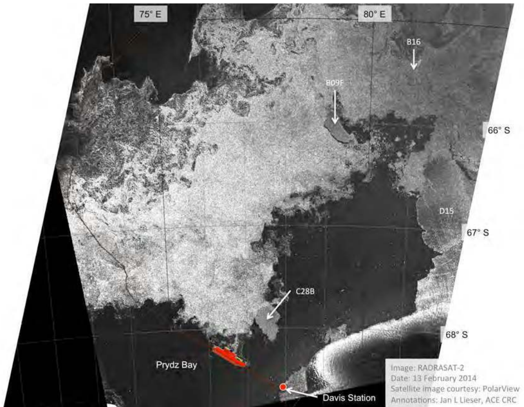
Figure 3: RADARSAR-2 image, acquired 13/02/2014 and provided by PolarView.
