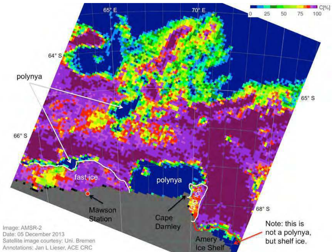
Figure 2: AMSR-2 image, acquired 05/12/2013 and provided by Universität Bremen.
