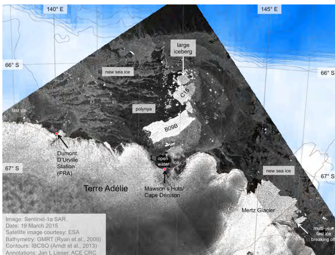
Figure 1: Sentinel-1a SAR scene, acquired 19/03/2015 and provided by PolarView.
