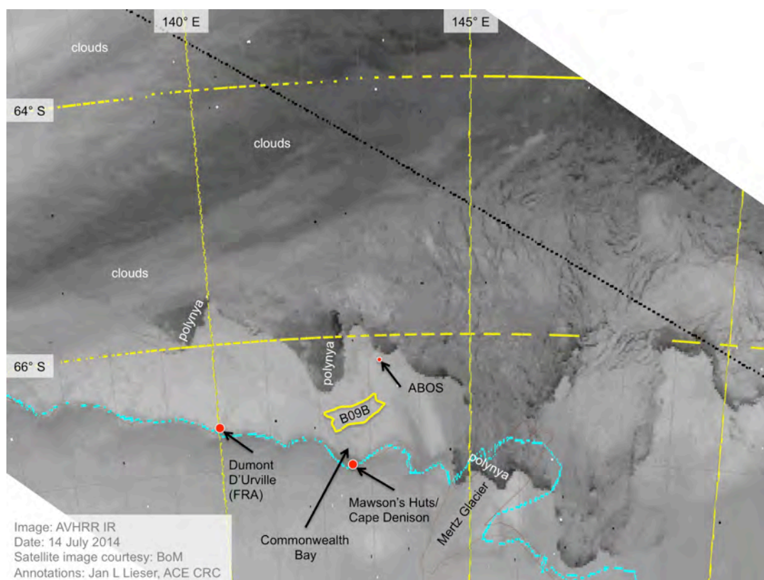
Figure 3: AVHRR image, acquired 14/07/2014 and provided by Bureau of Meteorology.
