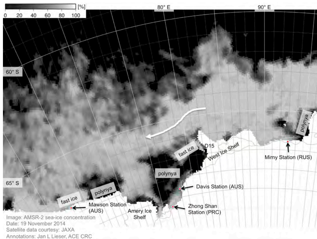
Figure 2: AMSR-2 image, acquired 19/11/2014 and provided by Drift &amp; Noise Polar Services.
