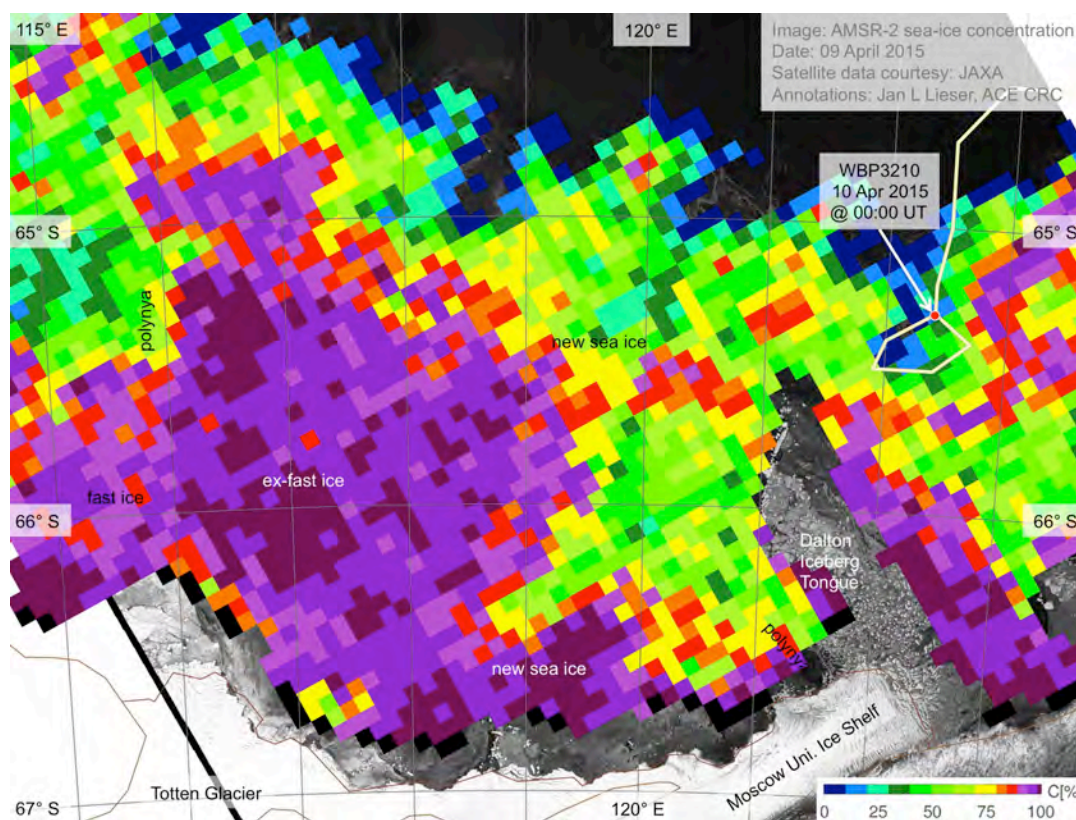
Figure 2: AMSR-2 sea-ice concentration map, acquired 09/04/2015 and provided by PolarView.
