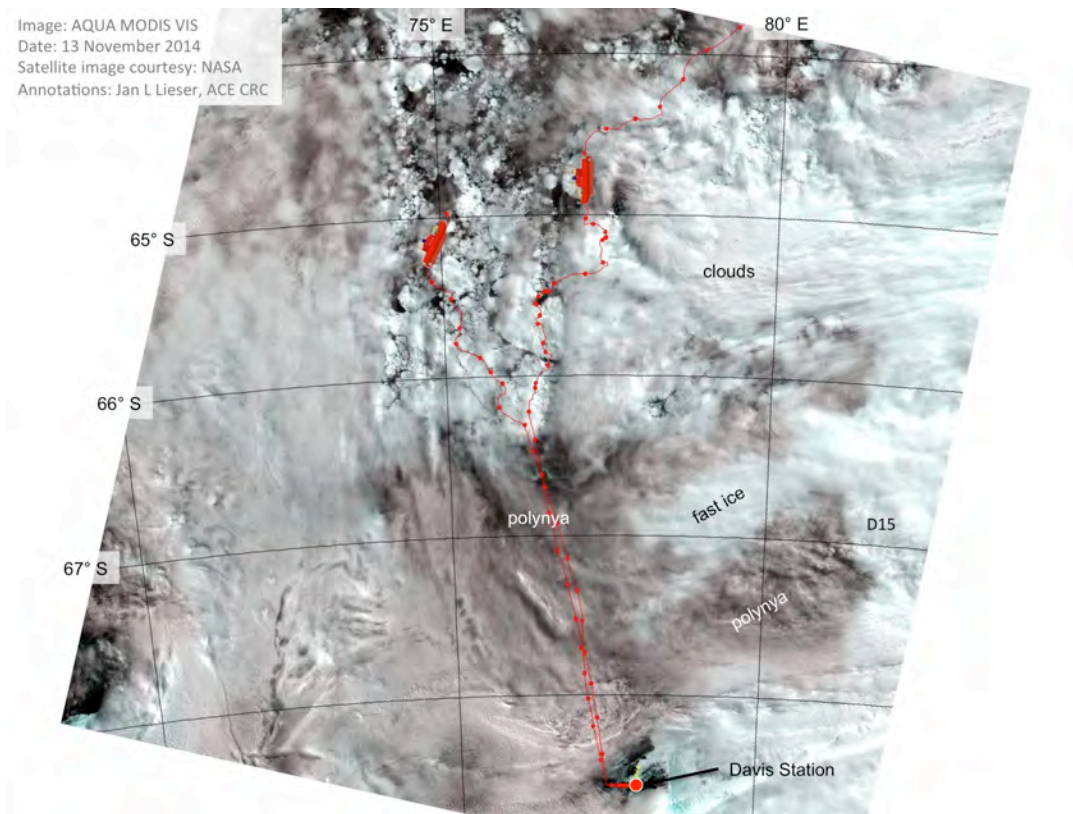
Figure 1: MODIS image, acquired 13/11/2014 and provided by NASA.
